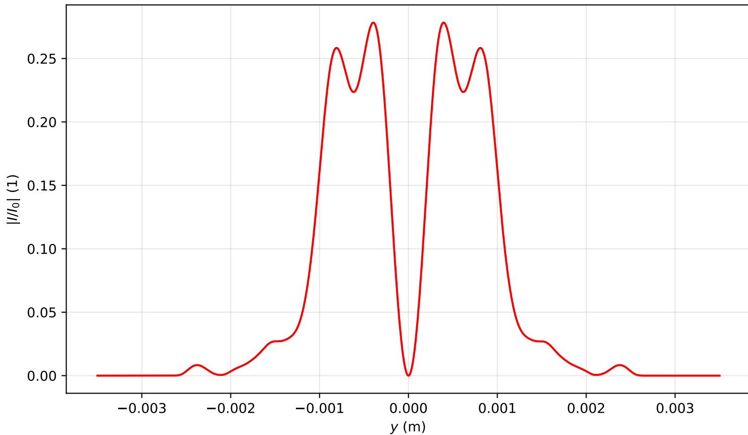
Intensity profile I(x=0, y, z=2.309)/I_0 , P_{in}=5.0P_{cr} , artificial time
